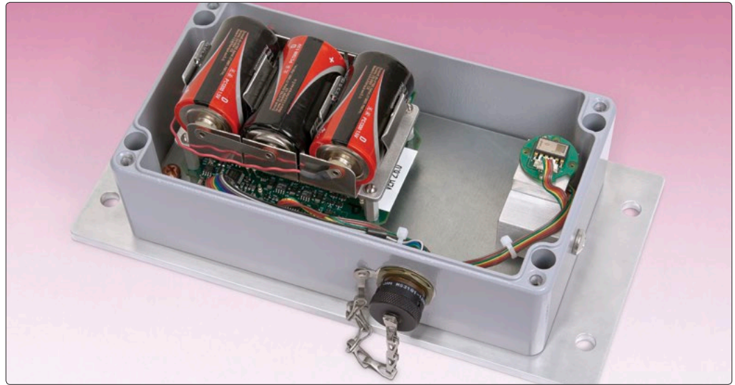
● Model 8003C-2 MEMS Datalogger shown with cover removed.
