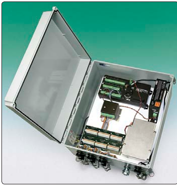
• Micro-1000 Datalogger.
