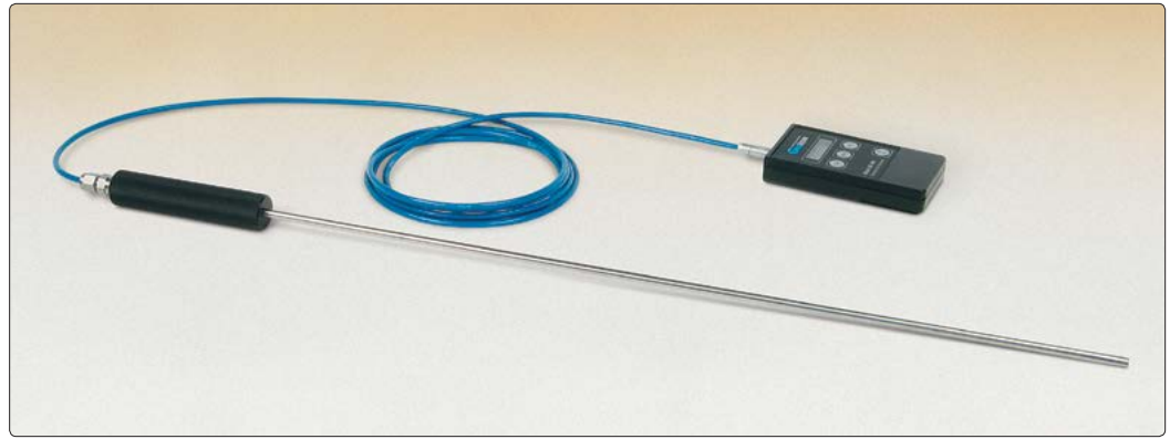
● Model 4910 Probe shown with the Model GK-404 Vibrating Wire Readout.
