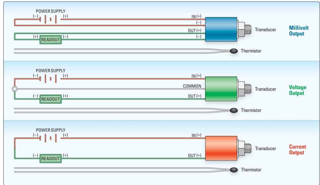
• Model 3400 Series Semiconducting Piezometer wiring schematics.
