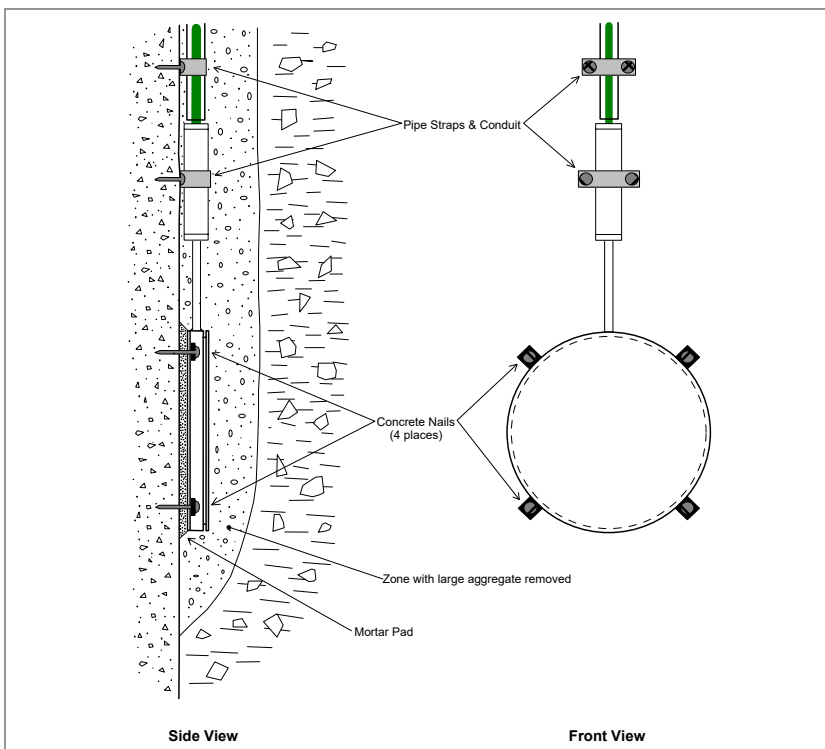
FIGURE 12: Model 4810 Contact Pressure Cell Installation
