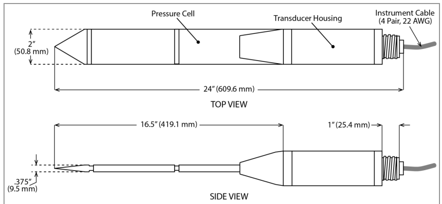
FIGURE 9: Model 4830 Push-In Pressure Cell
