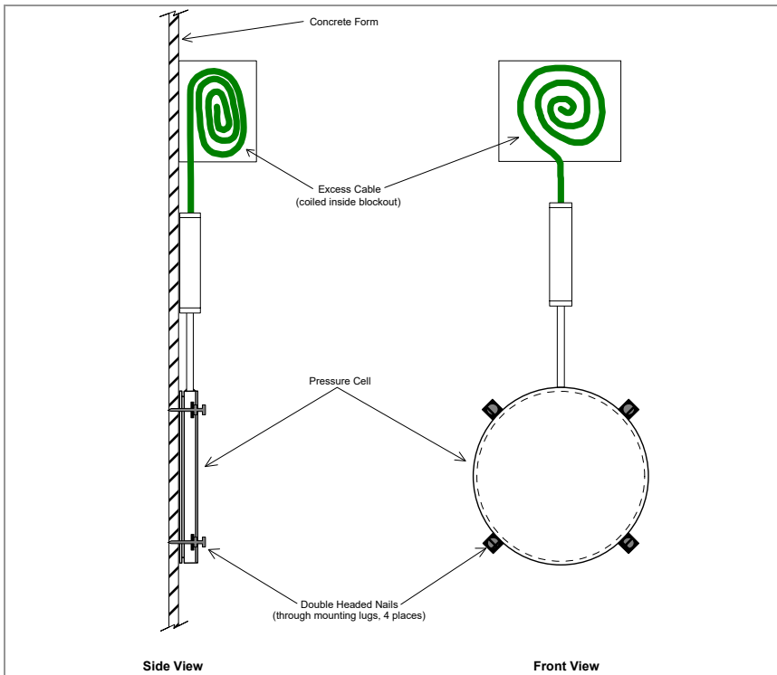
FIGURE 11: Attachment of Model 4810 to Concrete Form
