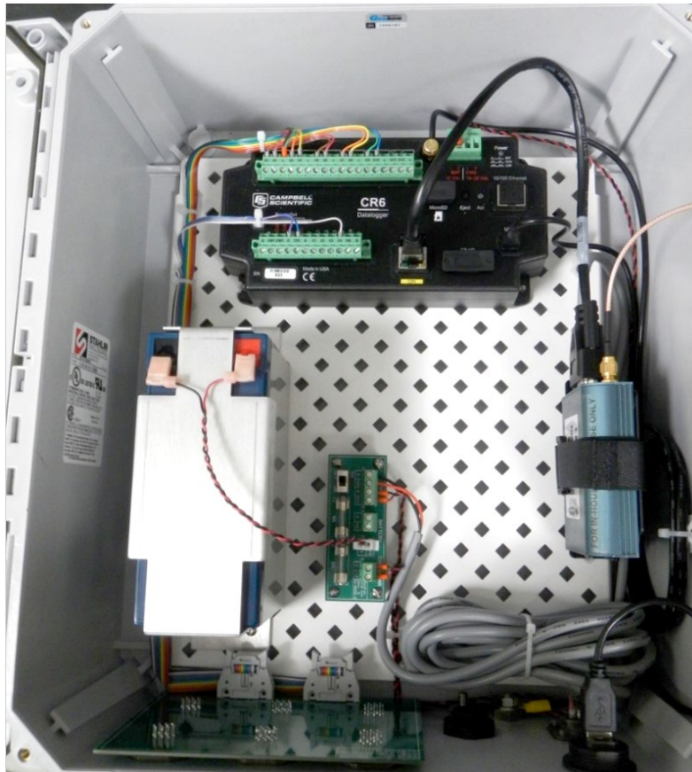
Figure 32 - Model 8600-1 with Cellular Modem Installed
