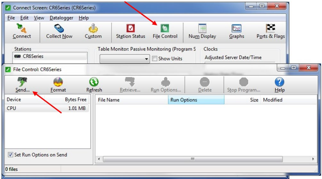
Figure 23 - Transfer File to Datalogger
