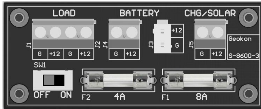
Figure 2 - Power Distribution Circuit Board
