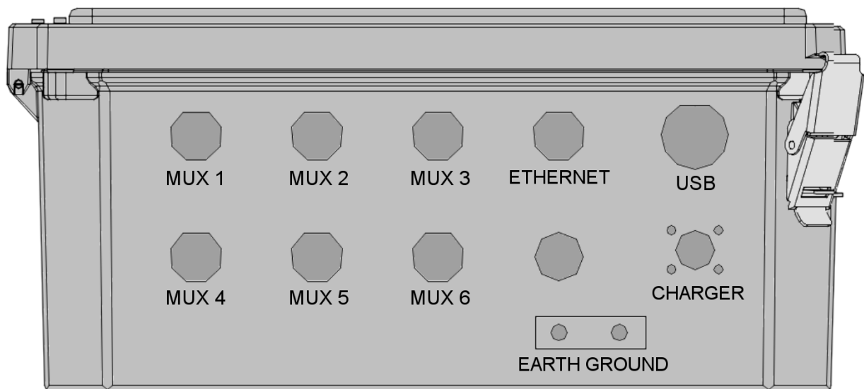
Figure 3 - Typical Bottom View MICRO-6000
