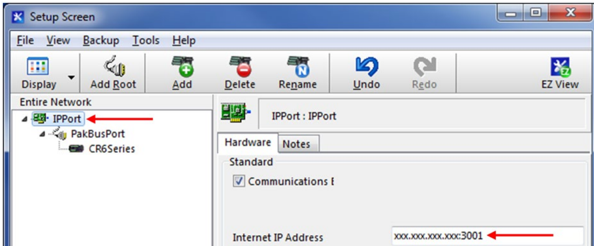
Figure 36 - Enter Internet IP Address
